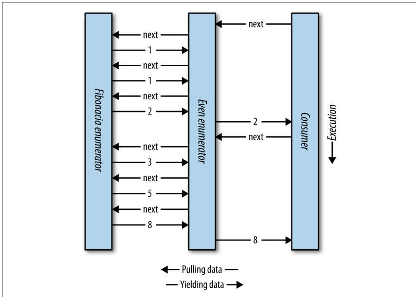
Figure 4-1. Composing sequences
