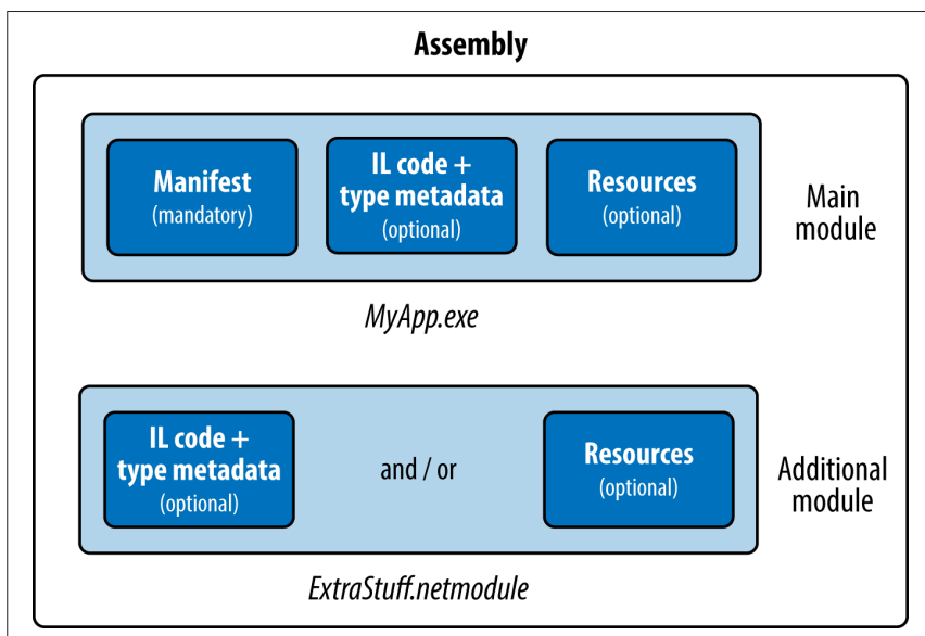
Figure 18-2. Multifile assembly
