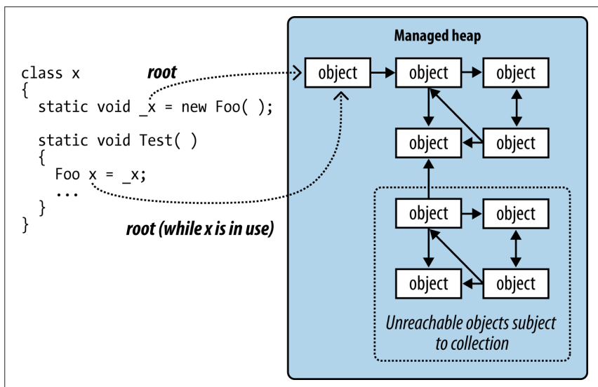
Figure 12-1. Roots
