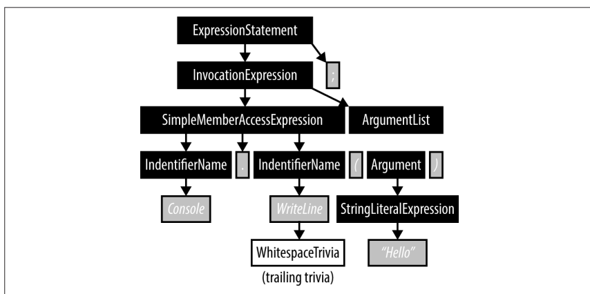
Figure 27-1. Syntax trees
