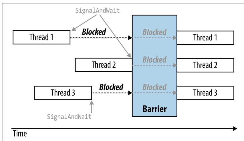
Figure 22-3. Barrier
