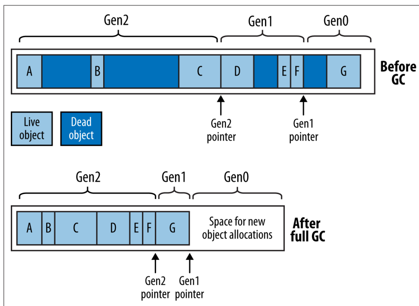
Figure 12-2. Heap generations
