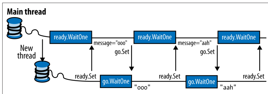
Figure 22-2. Two-way signaling
