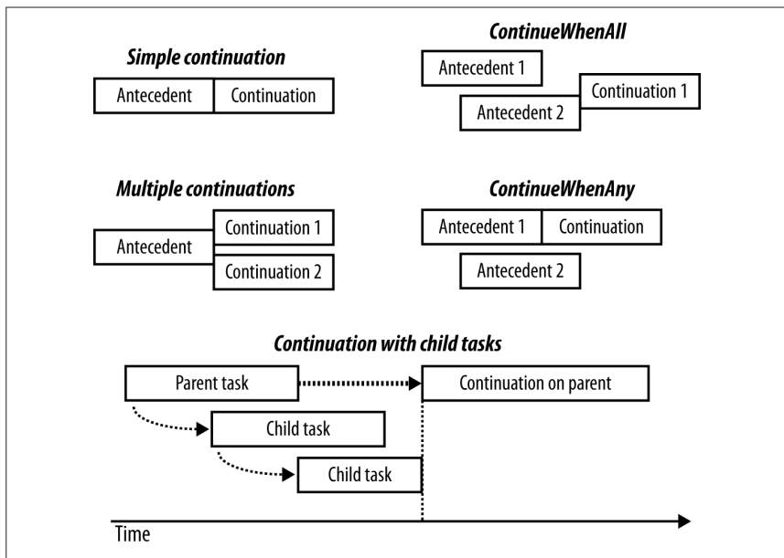
Figure 23-5. Continuations
