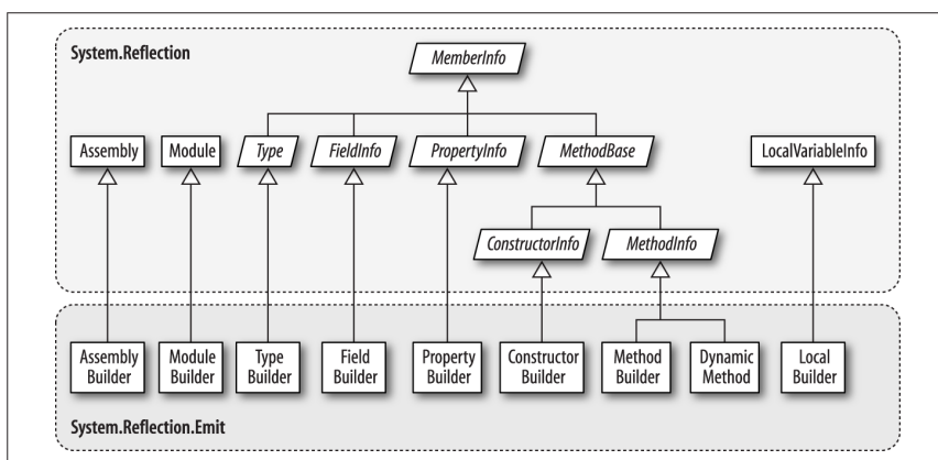
Figure 19-2. System.Reflection.Emit
