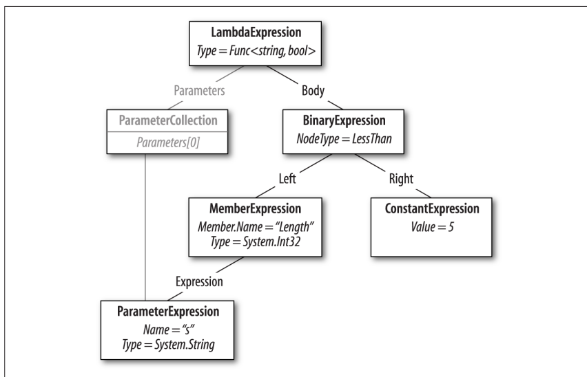
Figure 8-11. Expression tree
