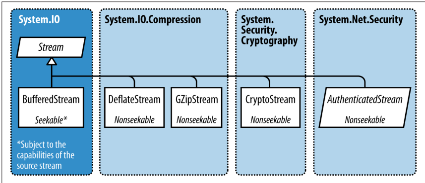
Figure 15-4. Decorator streams
