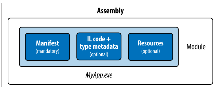
Figure 18-1. Single-file assembly
