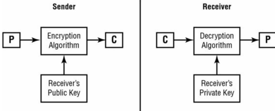
Figure 6.4 Asymmetric key cryptography
