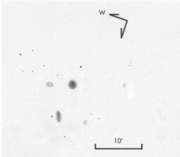
Figure 15.9 Galaxy grouping Hickson93 seen through a 300 mm scope. © Laurence Hall
