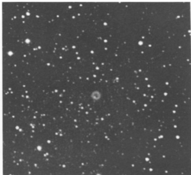
Figure 14.17 NGC6894, a perfect ring-structure planetary in Cygnus. © Nick Hewitt
