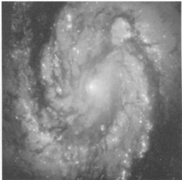
Figure 12.6 Grand-design spiral galaxy M100, from the HST. © STScI/NASA
