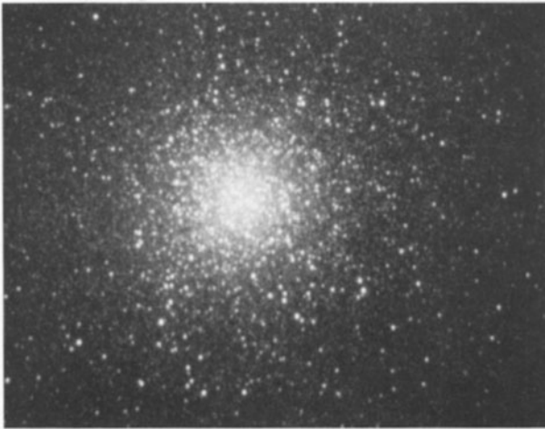
Figure 13.1 M13 in Hercules. Image autoguided using Starlight STAR software. © Terry Platt
