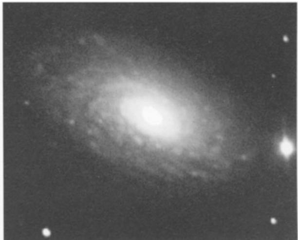
Figure 12.2 M63, the Sunflower Galaxy in Canes Venatici. © Grant Privett
