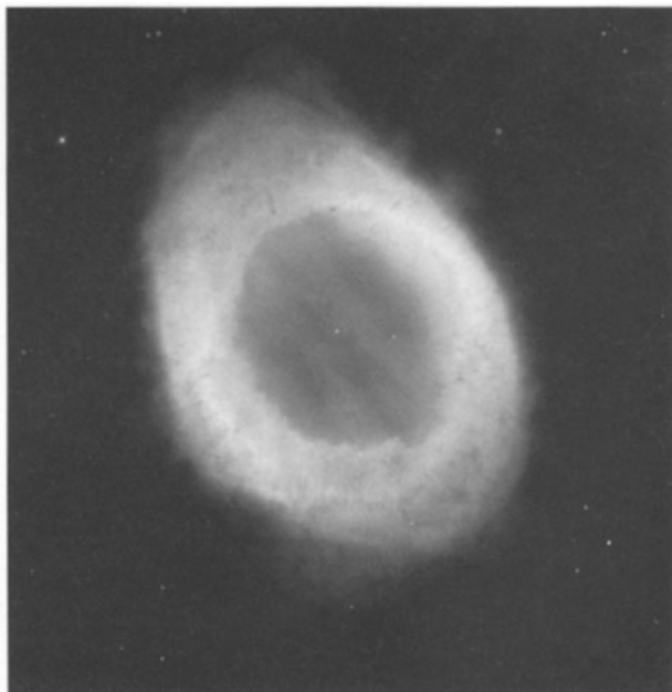
Figure 14.3 The Ring Nebula imaged by the Hubble Space Telescope. © STScI/NASA
