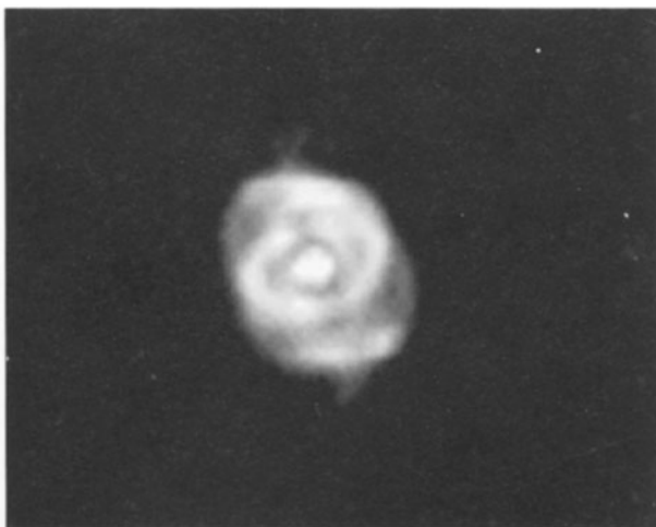
Figure 13.7 Fine detail within the Cat's Eye Nebula NGC6543. © Paul Curtis
