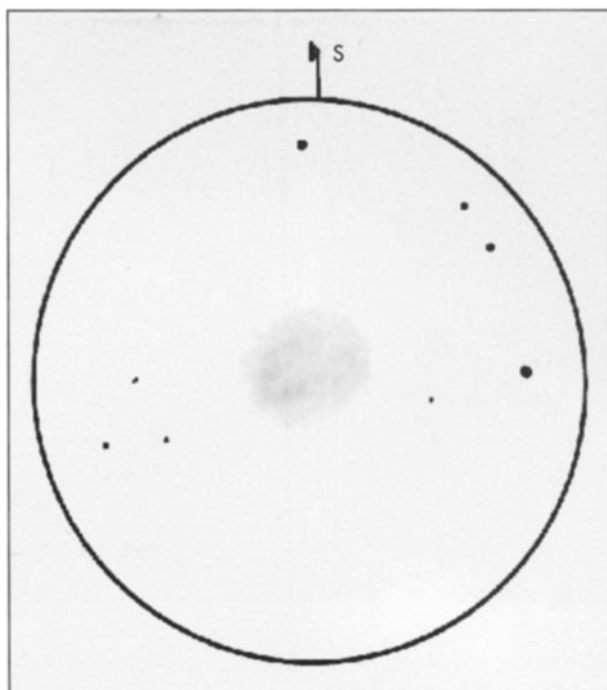
Figure 10.6 Easy to locate but tough to see. Local Group galaxy Leo 1. Tel: 20" F4.5. Eyepiece: 18 mm. Mag: \times 153 . Seeing: II. Filter: None. Field: 20'. © Stewart Moore
