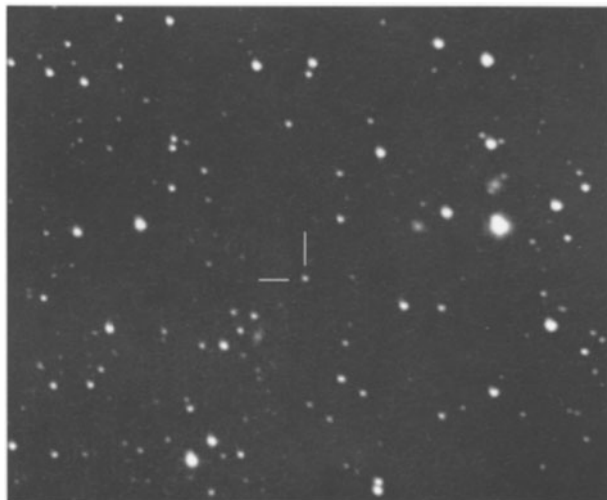
Figure 17.9 3C66A, an AGN monitored by the BAA. © Nick Hewitt
