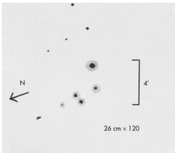
Figure 8.5 Nebulosity and cluster NGC2174/5 as seen in a 260 mm. © Guy Hurst
