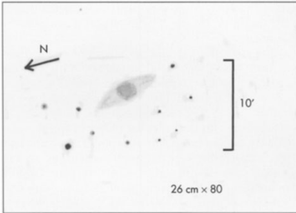
Figure 11.6 The galaxy NGC4656 in Canes Venatici using a 260 mm scope. © Guy Hurst
