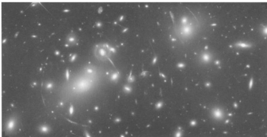
Figure 5.13 The Hubble Space Telescope's view of galaxy cluster Abell 2218. © STScI/NASA
