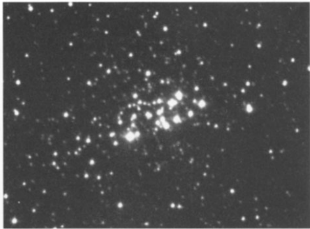
Figure 16.6 Small, compact and pretty – NGC 7510 in Cepheus. © Grant Privett
