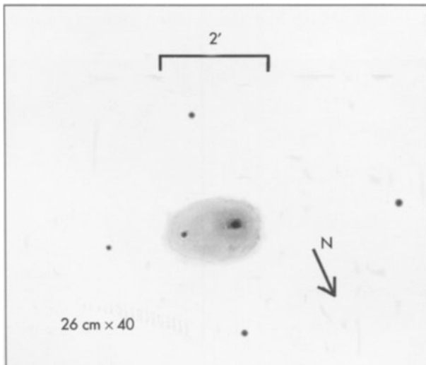
Figure 11.7 A drawing of Virgo galaxy NGC4608 using a 260 mm scope. © Guy Hurst
