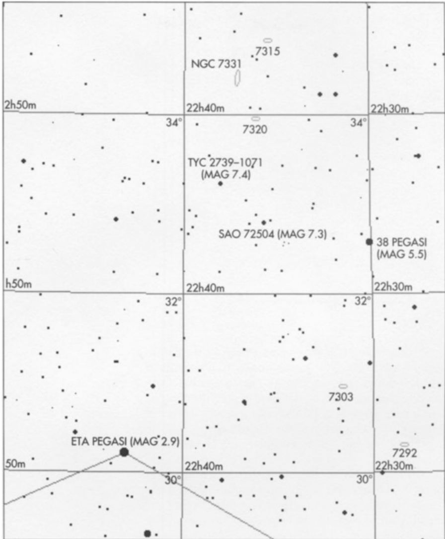
Figure 16.1 Finder chart for NGC7331. Courtesy SkyMap Software
