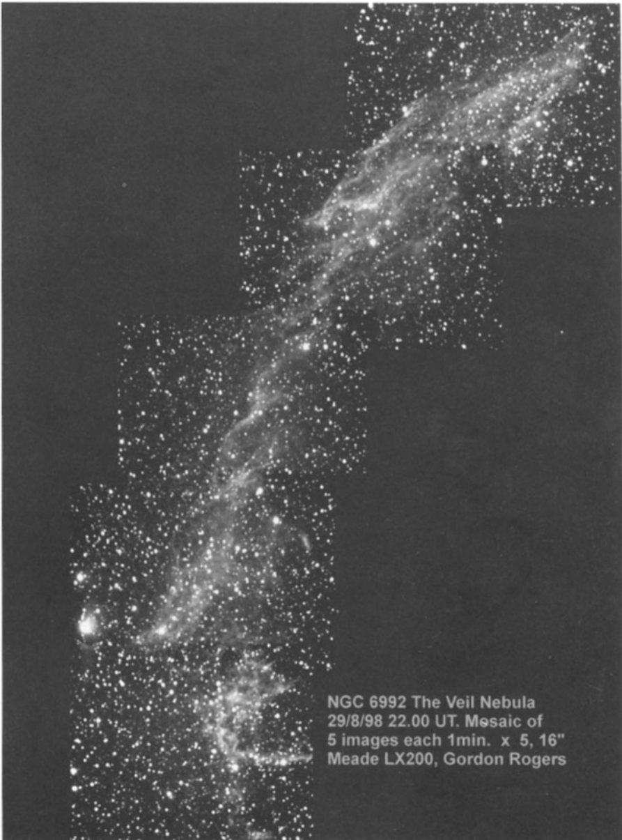
Figure 15.6 A mosaic of the intricate Veil Nebula in Cygnus. © Gordon Rogers
