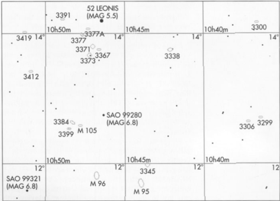
Figure 10.4 Finder chart for M95 and M96. Courtesy SkyMap Software
