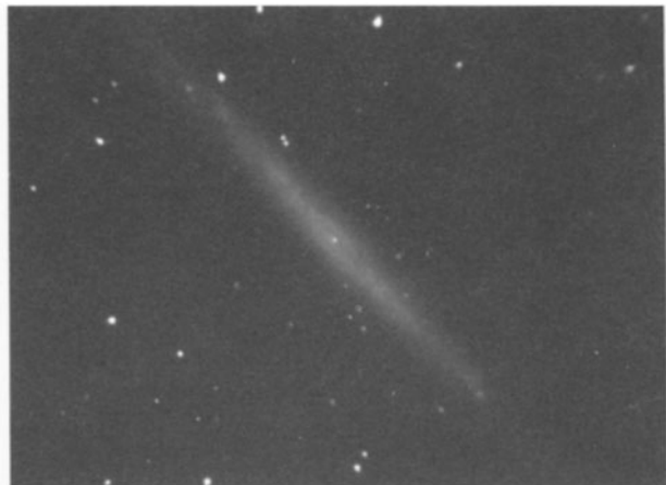
Figure 11.5 NGC4244 in Canes Venatici. © Peter Ward
