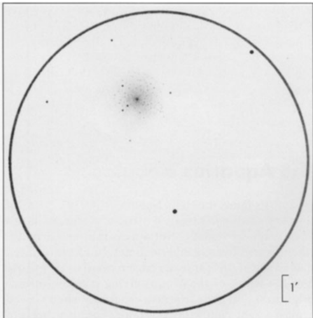
Figure 15.4 The often overlooked M15 in Pegasus. © Lee Macdonald
