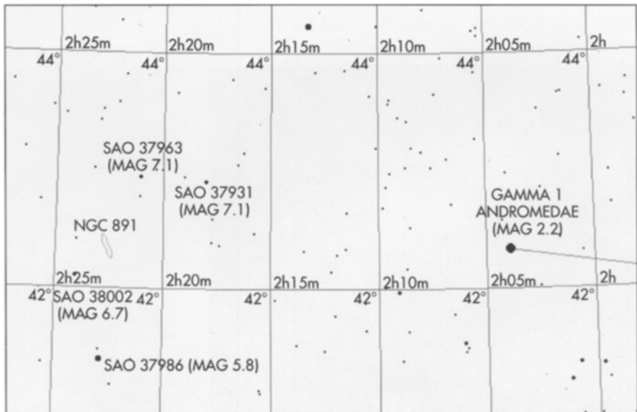
Figure 17.8 Finder chart for NGC891. Courtesy SkyMap Software
