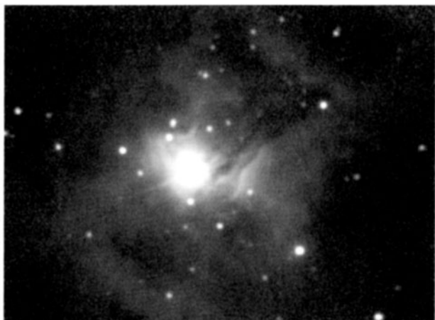
Figure 1.1 NGC7023, a lovely reflection nebula in Cepheus. © Grant Privett
