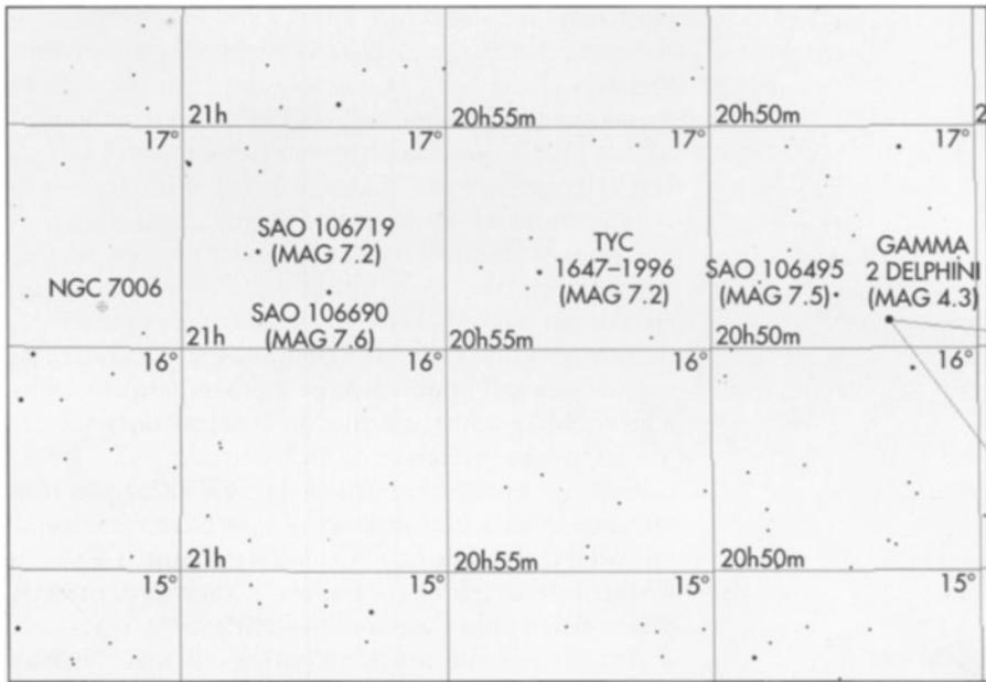
Figure 14.9 Finder chart for NGC7006. Courtesy SkyMap Software
