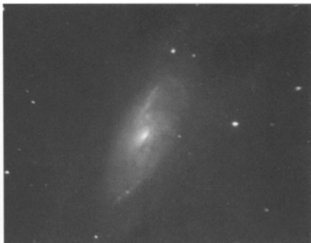
Figure 10.10 M106, an inclined spiral galaxy in Canes Venatici. © Peter Ward
