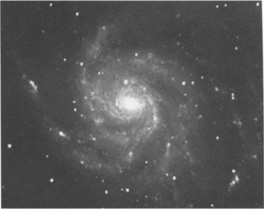
Figure 12.1 M101, its arms a mass of knotty condensations and HII regions. © Nik Szymanek
