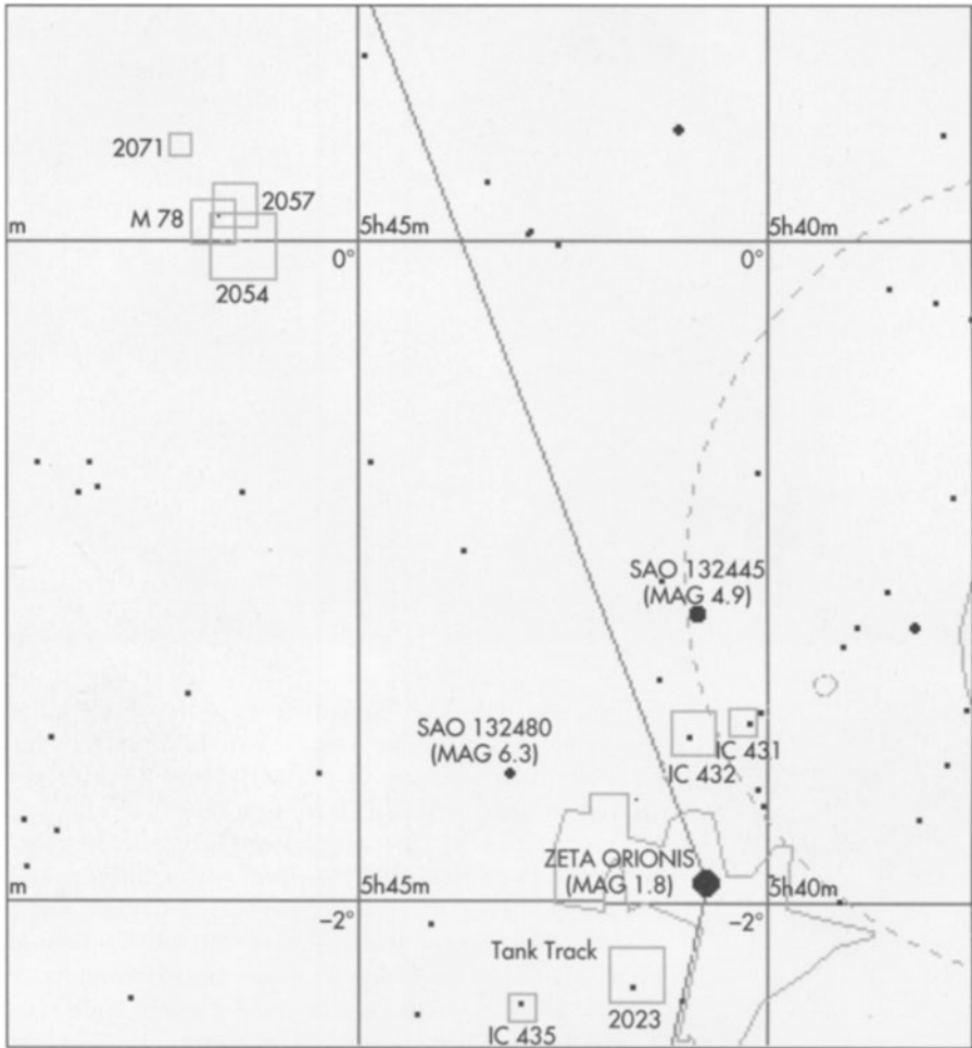
Figure 19.8 Finder chart for M78. Courtesy SkyMap Software
