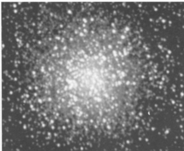
Figure 14.12 M22: A grand globular cluster in Sagittarius. © Mike Fleenor
