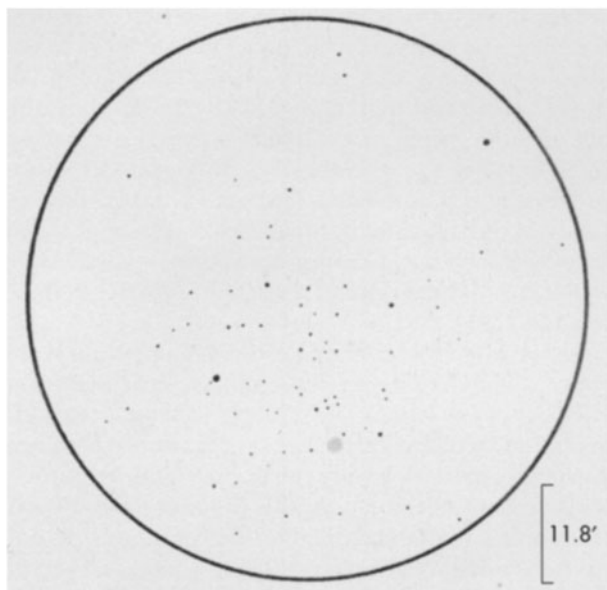
Figure 8.4 NGC2438 nestling on the edge of M46 in Puppis. © Lee Macdonald
