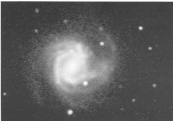
Figure 11.1 M61, a spiral galaxy in Virgo. © Grant Privett
