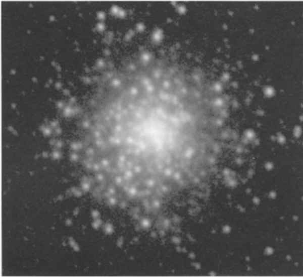
Figure 15.5 M15, a globular cluster in Pegasus. © Grant Privett
