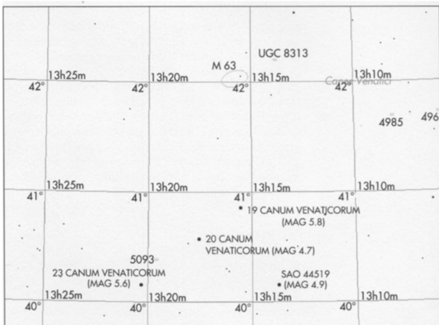
Figure 12.4 Finder chart for M63. Courtesy SkyMap Software
