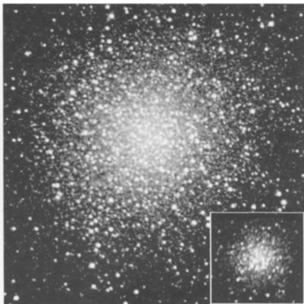
Figure 5.17 M13 and NGC2419 to the same scale. © Maurice Gavin
