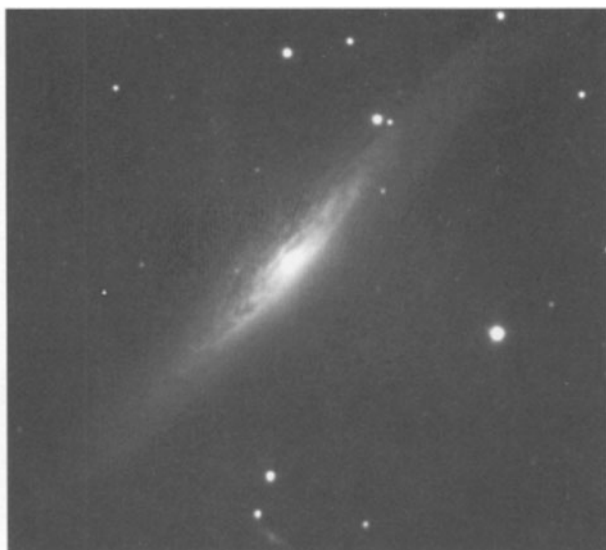
Figure 9.9 The galaxy NGC2683 in Lynx. © Gordon Rogers
