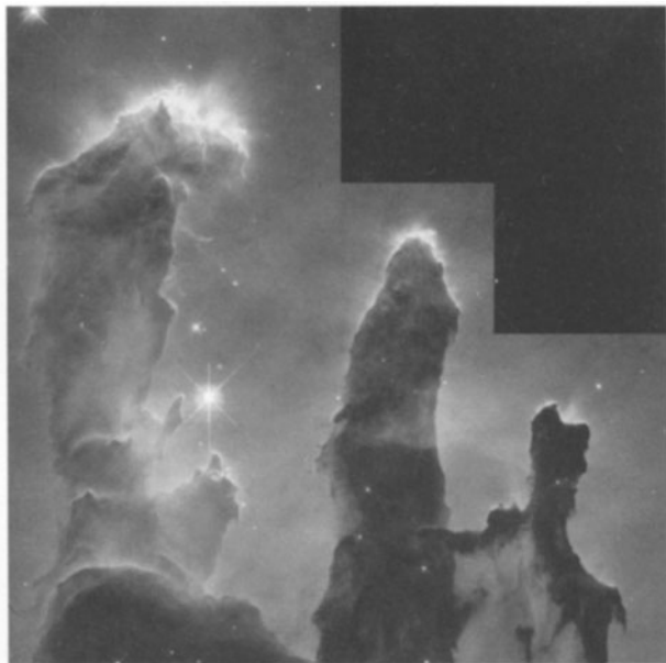
Figure 14.14 Dark nebulae in the Eagle Nebula, M16. © STScI/NASA
