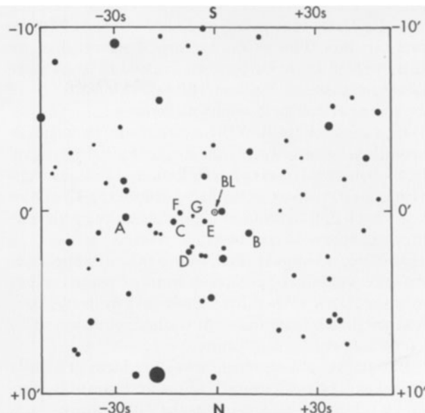
Figure 5.22 Finder chart for BL Lacertae.
