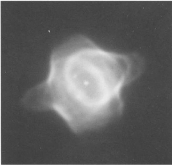
Figure 5.15 The Stingray is the youngest known planetary nebula. © STScI/NASA
